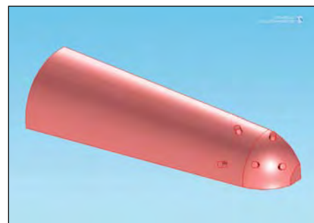
Fig. 1. A quarter symmetry of the actual nozzle geometry with a typical placement of holes modeled in COMSOL (right)
