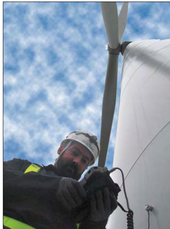
Brett monitoring vibration of a wind turbine tower with a hand held accelerometer.
