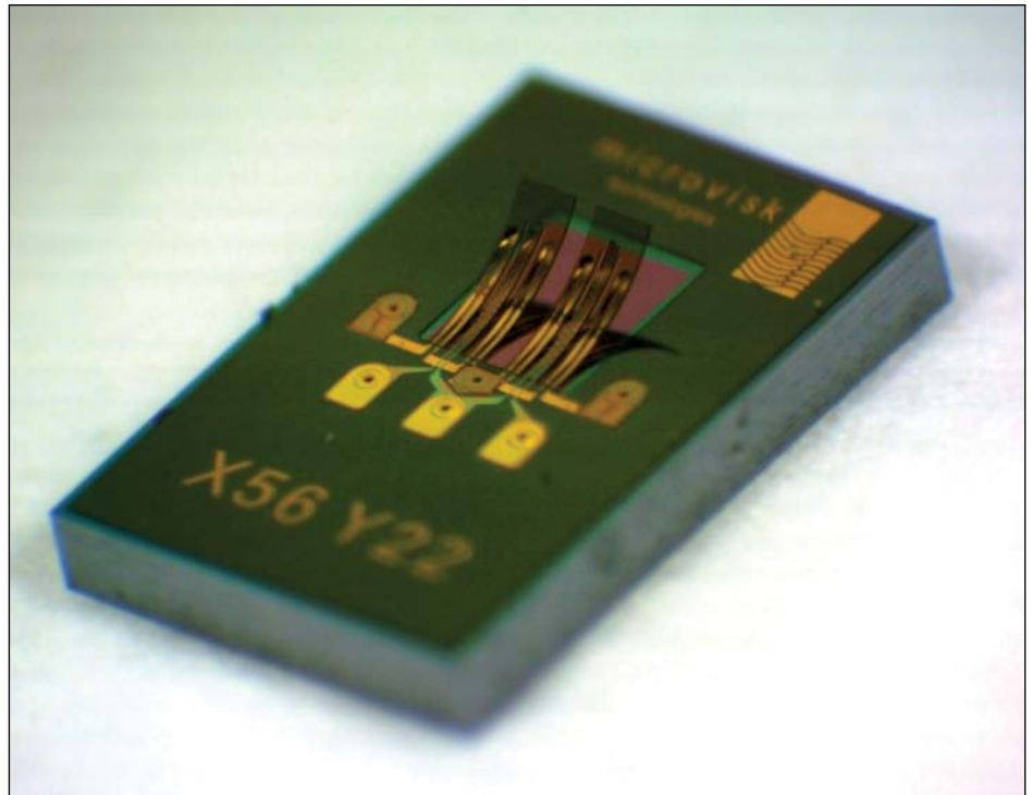
Figure 1. Microvisk's MEMS-based micro-cantilever device.
