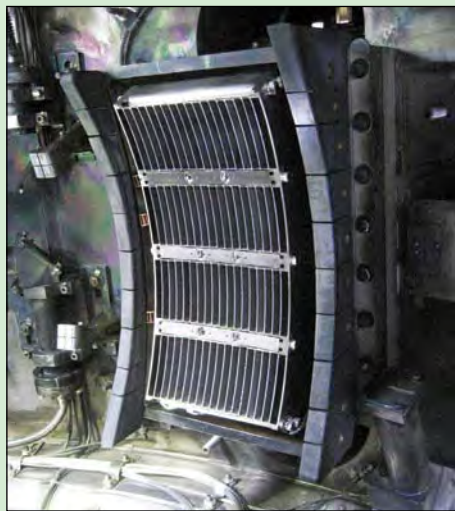
Lower hybrid grill antenna as seen from inside of the Alcator C-Mod vessel. The arrays of open-ended waveguides are phased so to launch the waves preferentially in one toroidal direction, so accelerate electrons and ultimately drive current inside of the plasma.
