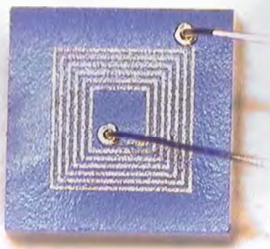
Fig. 1. Image of a \mu MS coil. The typical overall dimensions of the coils are 350 \mu\text{m} \times 350 \mu\text{m} .
