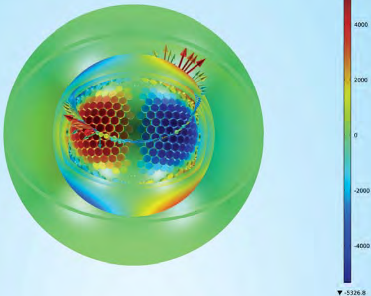
Fig. 3. Radial magnetic flux density at the rotor surface (surface plot) and magnetic flux density (arrow plot).
