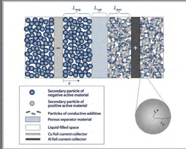
Figure 1. Diagram showing the basic components of a battery. The (+) and (-) refer to the positive and negative terminals, respectively. The simulation equations are solved in the two dimensions ( x and r ) throughout the negative electrode, separator, and positive electrode domains, denoted by L_{neg} , L_{sep} , and L_{pos} , respectively.
